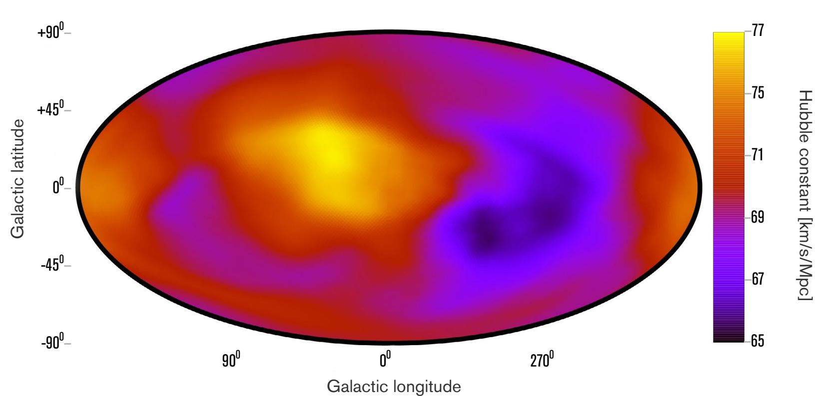
All-sky map showing what may be a lopsided expansion of the universe, based on x-ray surveys of hundreds of galaxy clusters. Orange-yellow hues indicate a faster-than-expected expansion rate. Purple-black colors correspond to slower-than-expected expansion.
